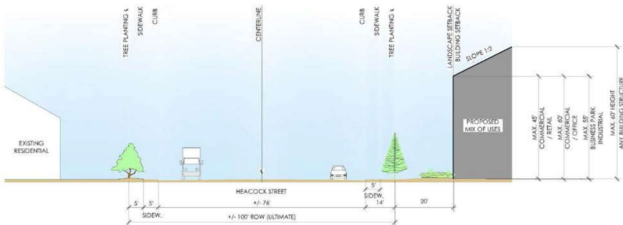
Figure 4-10 Heacock Street Section D
