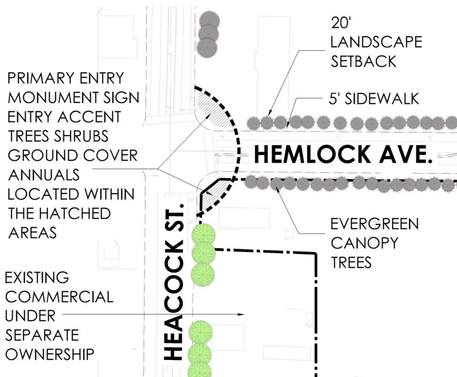
Figure 4-25 Entry Plan
