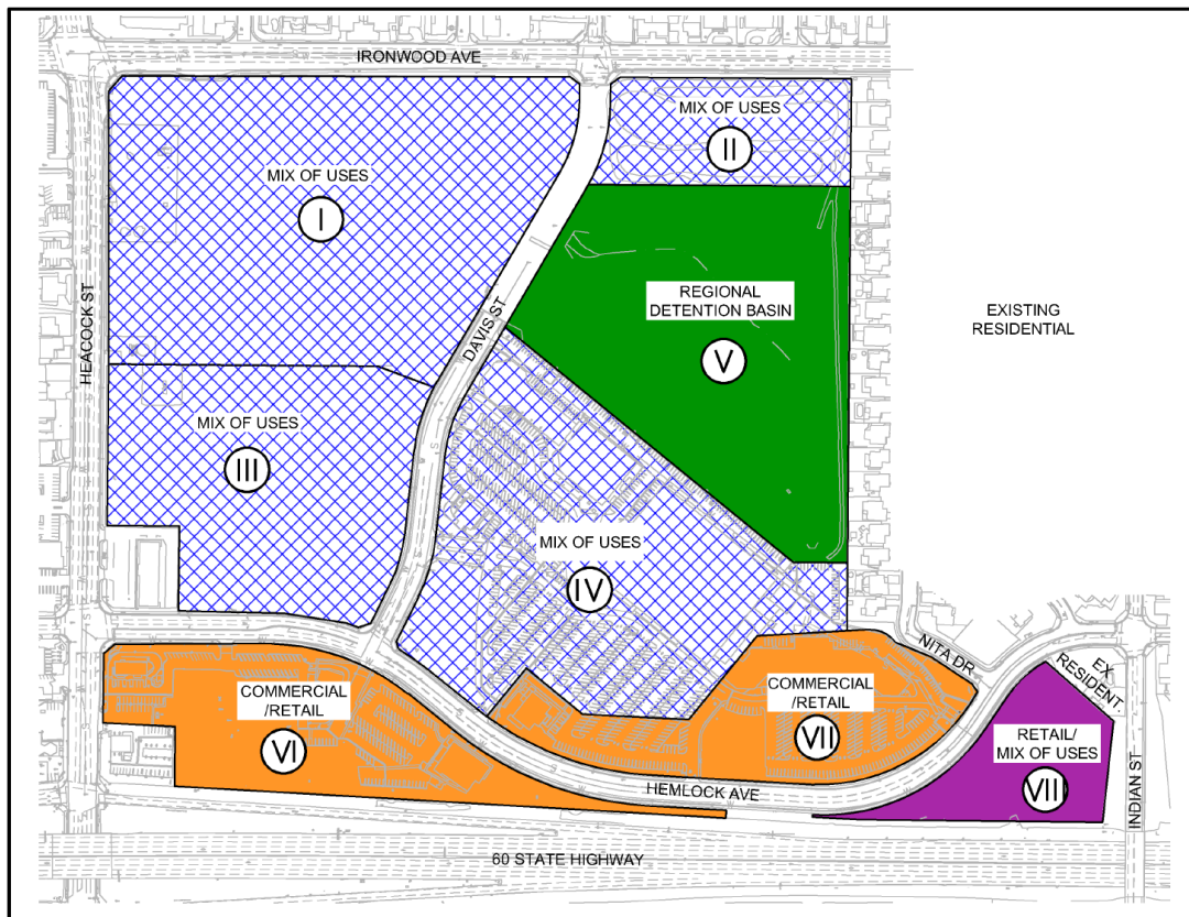
Figure 2-1 Land Use Plan
